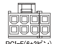
PCI-E(6+2ピン)
