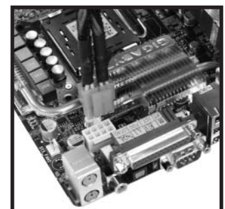
EPS12V(4+4ピン)
