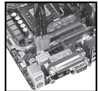
EPS12V(4+4ピン)
