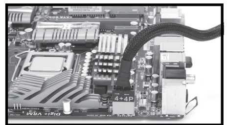
EPS12V(4+4ピン)
