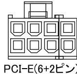
PCI-E(6+2ピン)
